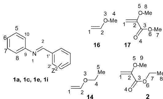
Fig. 3 Structures and numbering considered in the 13 C NMR and computational modelling. The dihedral angles \theta_i , reported in Table 6 are defined according to: \theta_1 = (10, 9, 1, 2) , \theta_2 = (1, 2, 1', 2') and \theta_3 = (10, 9, 1', 2') for imines 1 and \theta_1 = (1, 2, 3, 4) for compounds 16 and 17 .
