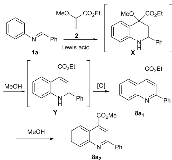
Scheme 2 Postulated intermediates in the reaction of imine 1a with acrylate 2 .
