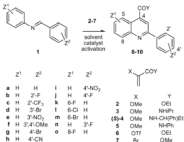
Scheme 1 Reaction of imines 1 with 2-substituted acrylic acid derivatives 2–7 .
