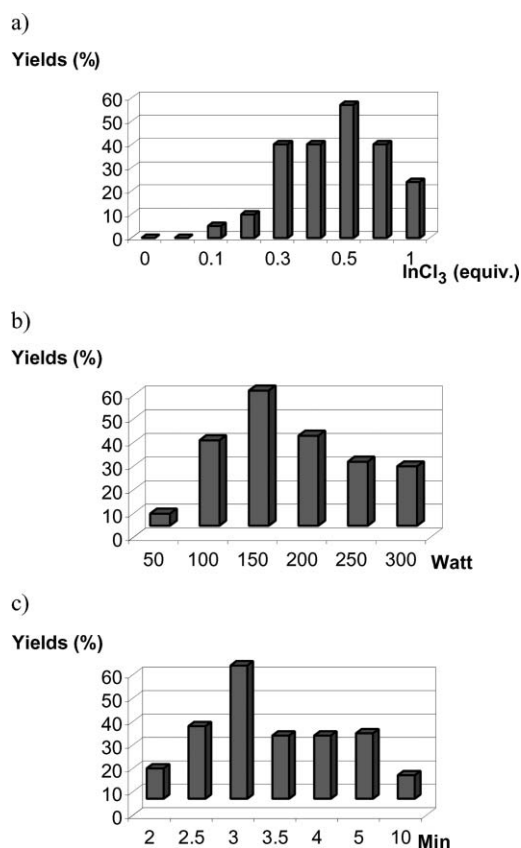
Fig. 2 Reaction of imine 1a with acrylate 2 . Yields as a function of (a) amount of InCl 3 , (b) power of microwave irradiation, (c) reaction time.
