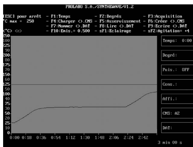
Fig. 4 Temperature (°C) as a function of time (min) inside the microwave oven (irradiation power: 150 W).
